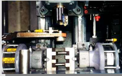
Face & Chamfer Tool with clamp
